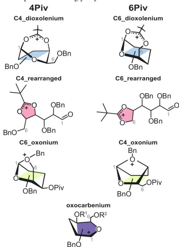
Scheme 1. Structures that can be adopted by (left) 4Piv and (right) 6Piv galactosyl cations. Oxocarbenium structures can be adopted by both cations. Except for oxonium structures, all five structures can be adopted by 4,6Piv .
