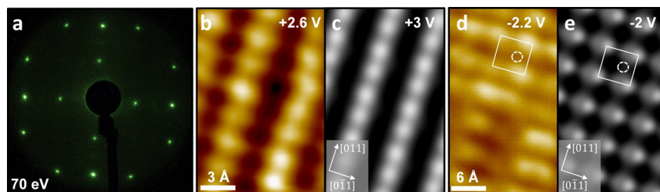
Figure 3. a) LEED pattern (70 eV electron energy) and b), d) high-resolution STM images of a reduced \text{Co}_3\text{O}_4(100) film. Image (b) was recorded with a positive +2.6 V and (d) with a negative -2.2 V sample bias voltage. c), e) STM simulations (DFT + U ) for B-layer terminated \text{Co}_3\text{O}_4(100) with one Vac( \text{O}_{30} ) per unit cell for positive and negative sample bias voltages. The surface unit cell and the position of the \text{O}_{30} oxygen vacancy (open circle) are indicated in (e).
