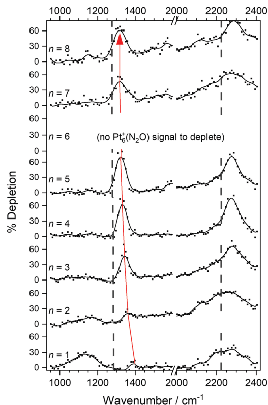
Fig. 4 IR-MPD spectra of \text{Pt}_n(\text{N}_2\text{O})^+ ( n = 1-8 ) clusters recorded in depletion of the parent cluster ion. The dashed lines at 1285\text{ cm}^{-1} and 2224\text{ cm}^{-1} indicate the wavenumbers of the \text{N}=\text{O} and \text{N}=\text{N} stretches of free \text{N}_2\text{O} , respectively. 50
